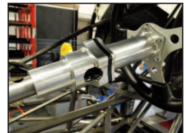
Quick Release Stabilizer and Extension
